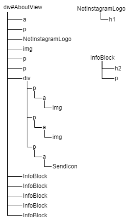
Figure 5: Graphical subdivision of the About page into components
