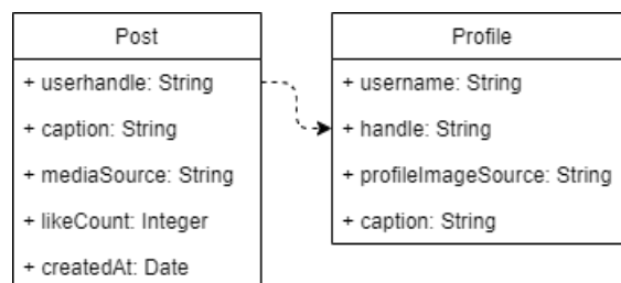
Figure 3: Classes used by the NotInstagram services
