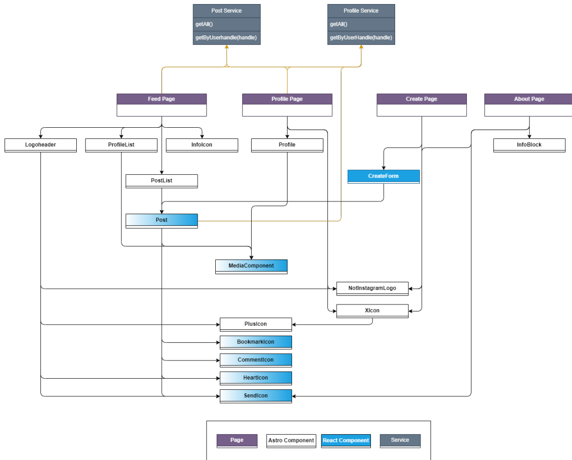
Figure 6: Adapted component structure for Astro Islands (React components are marked blue, duplicate components are white and blue)
